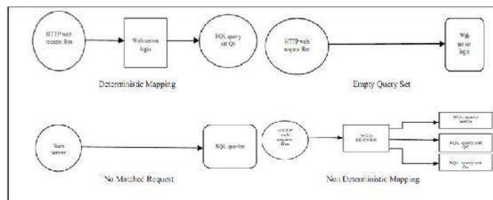
Fig 3: Mapping Pattern
