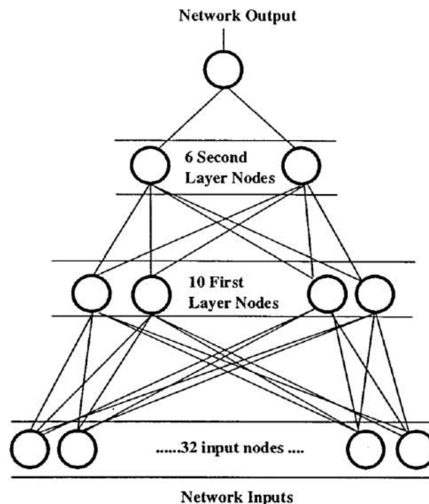
Figure.4.The network structure
