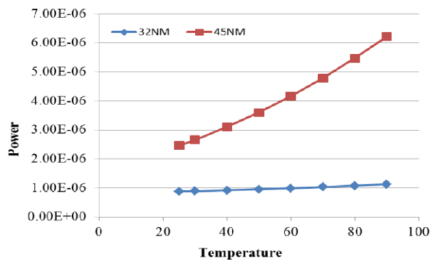
Figure 8. comparison of average power as function of temperature
