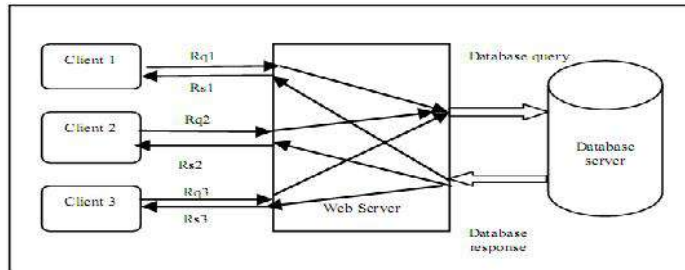
Fig 1: Classical Architecture of Three Tier System
