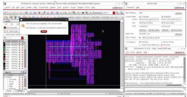
Fig.12. Layout and LVS match for Reversible Multiplier
