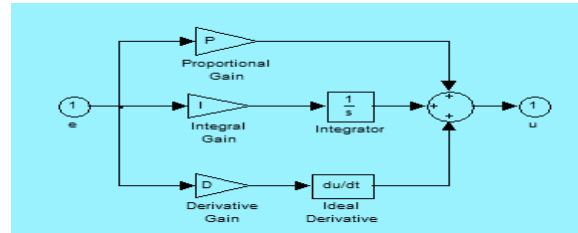
Fig.5. PID Control Scheme
