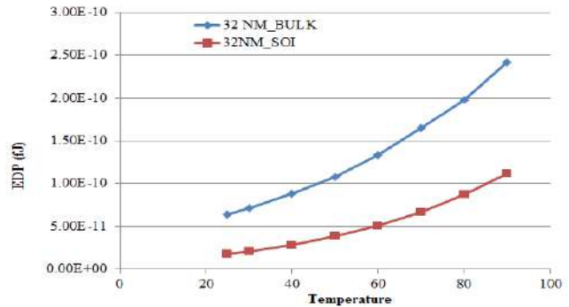
Fig. 9: Energy Delay product vs temperature
