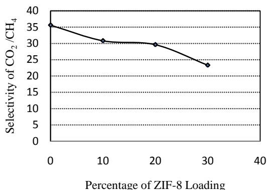
Fig.2. Effect of percentage ZIF-8 loading on selectivity CO 2 /CH 4 of PES–ZIF-8 MMM at 3 bar 30°C.
