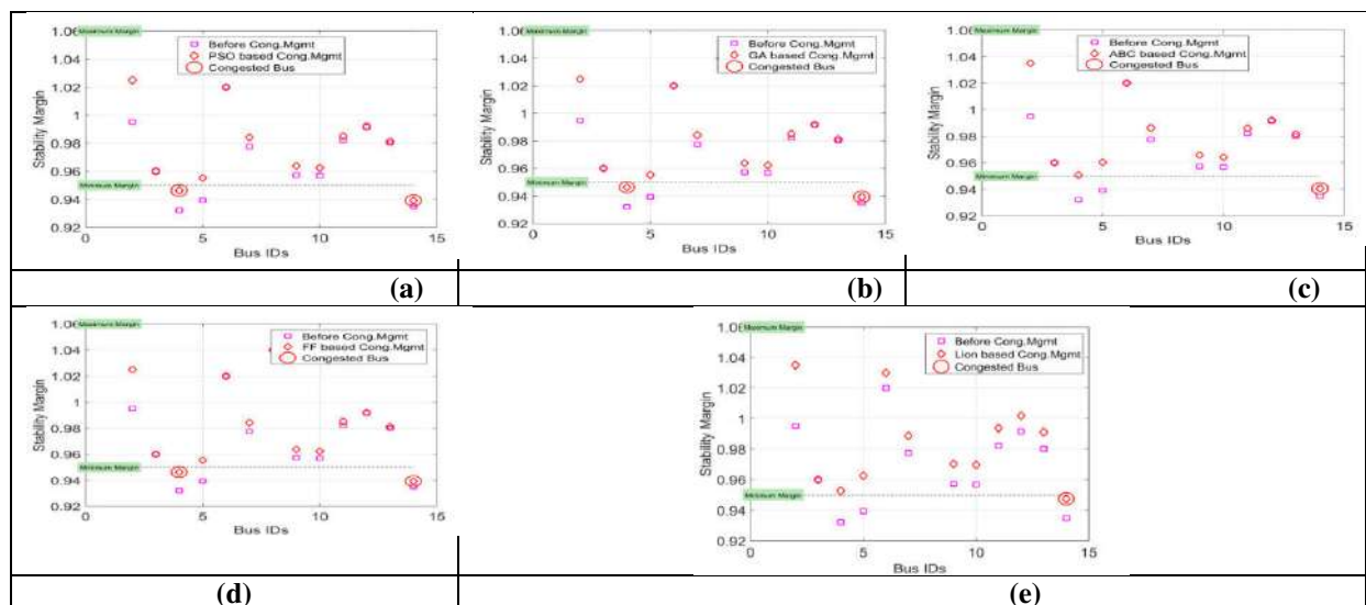
FIG. 3 DEMONSTRATION OF CONGESTION ANALYSIS BY PSO,GA,ABC,FF AND LA FROM IEEE BUS SYSTEMS (A),(B),(C),(D),(E) FROM IEEE 14 BUS SYSTEM
