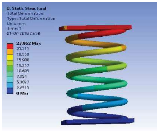
Figure 4. Total Deformation of Existing Compression Spring for 500 N Load
