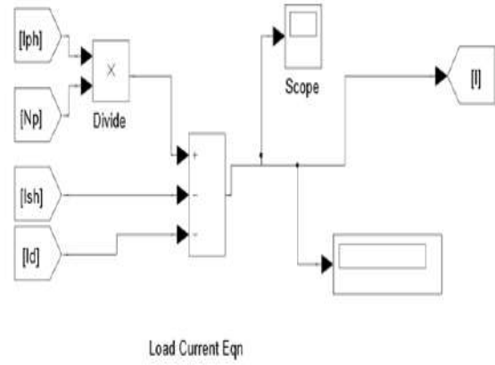
Figure 3: Simulink model for load current equation.
