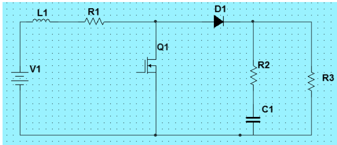
Fig. 2: Boost converter circuit
