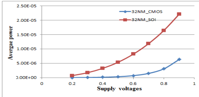
Fig. 5: Comparison of power as function of supply voltage
