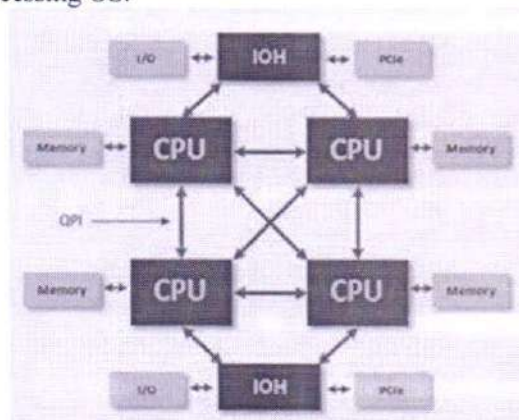
Fig.6: e. Multiprocessing Operating System
