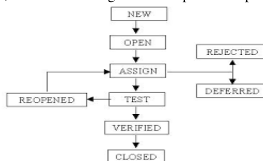
Figure 2: Defect Management Life Cycle
