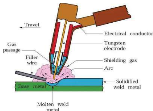
Fig-1.2 GTAW Welding Process
