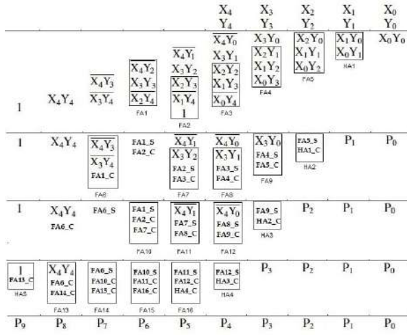
Fig.6. Multiplication by Wallace approach in the proposed circuit
