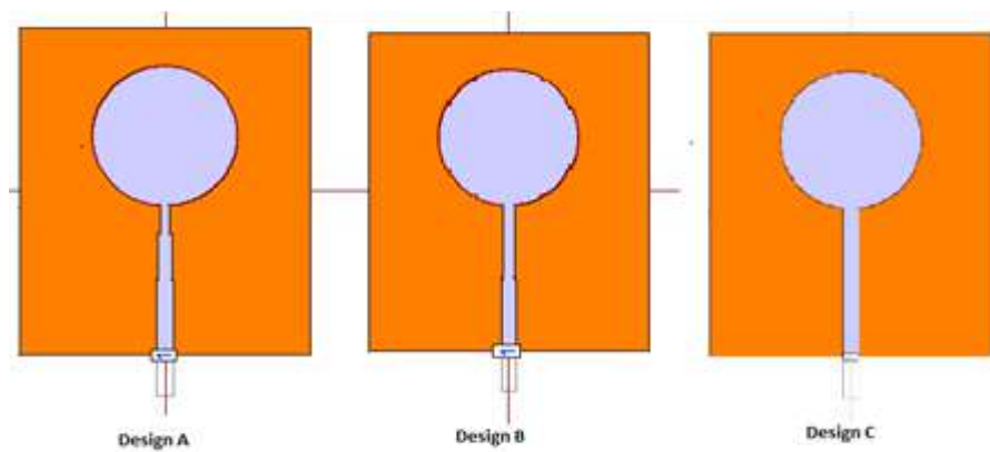
Fig(3): 3 Designs by using IE3D simulator
