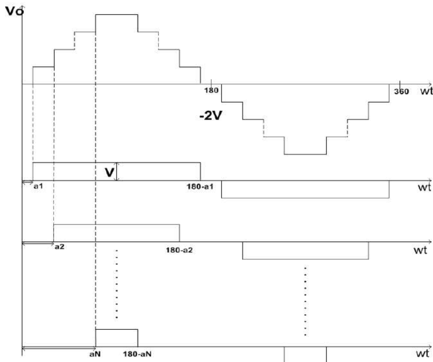
Fig. 2. Staircase output phase voltage of N level inverter
