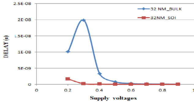
Fig. 4: Comparison of Delay as function of supply voltage
