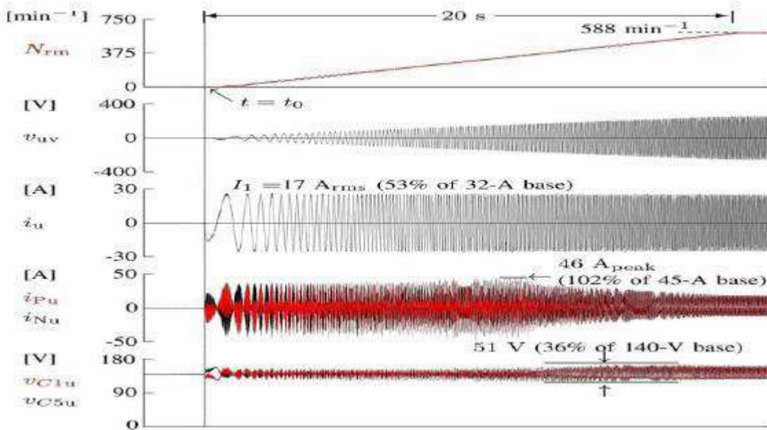
Fig 1: Experimental start-up waveforms when I^{**} = 17 A (53%), and T_l = 60\% , where I_0 = 12 A (65%).
