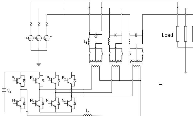
Fig. 2. Three-Phase Four-Wire DVR
