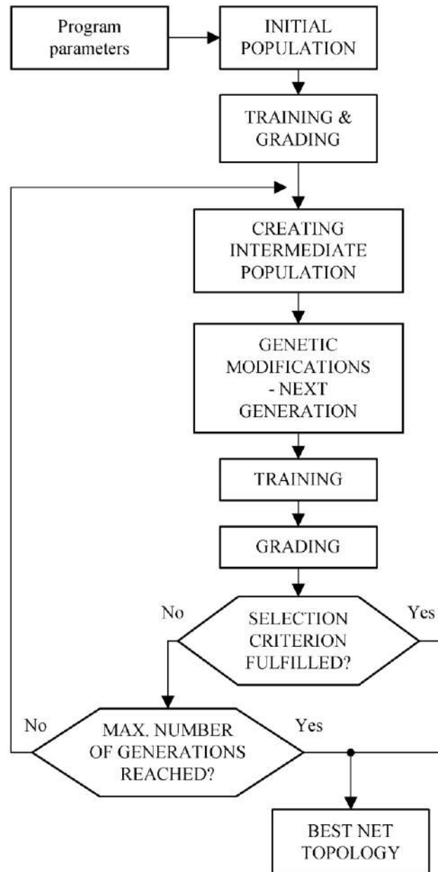
Figure.3. Flowchart of the GA procedure for the ANN topology optimization.
