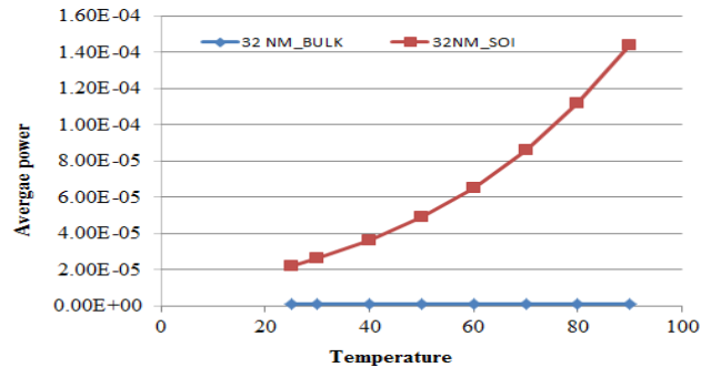
Fig. 8: Comparison of average power as function of temperature
