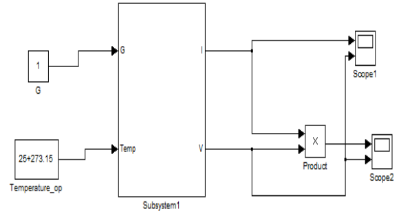
Figure 4: Simulink model of PV array module.
