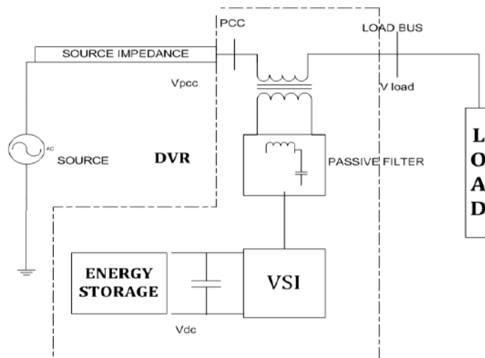
Figure 1: Basic Structure of A DVR
