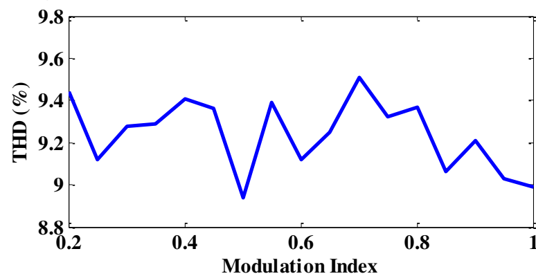
Fig. 5(a). THD verses modulation index for 5 level inverter
