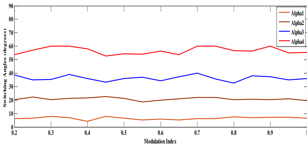
Fig. (4)(b). Modulation index verses switching angles for 9 level CHB
