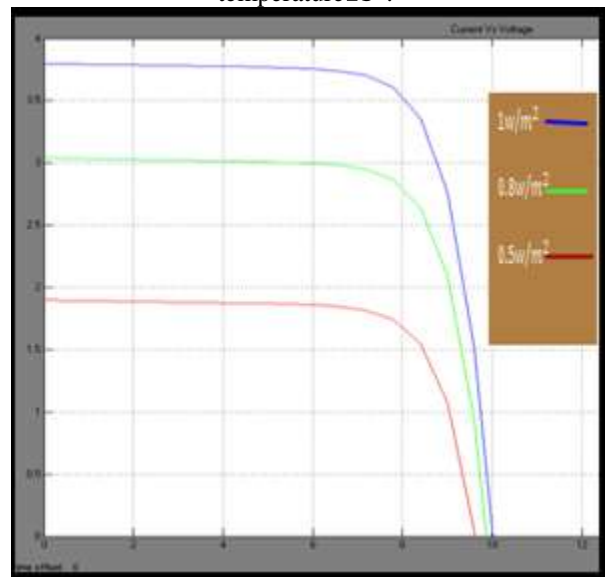
Figure 8: Effect of solar insolation on I-V curve at temperature 25^{\circ} .
