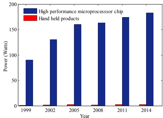
Figure 1. Power requirements of microprocessor chip and portable products as per ITRS [17-19].
