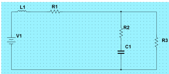
Fig.3: Top – MOS switch ON (diode in reverse bias) Bottom – MOS switch OFF (diode conducting)
