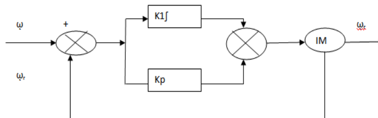
Figure 3. Block diagram PI controller
