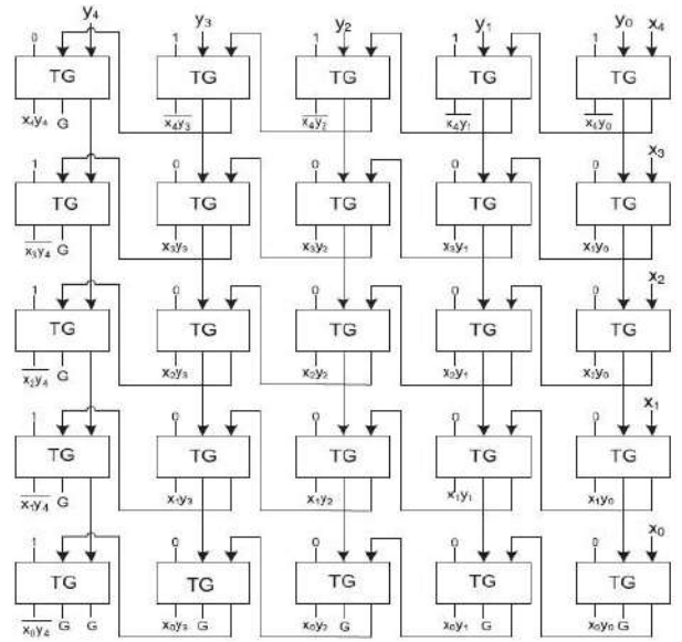
Fig.7. Partial Product Generation by Toffoli Gates
