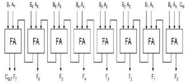
Fig. 3: 8-bit Ripple Carry Adder
