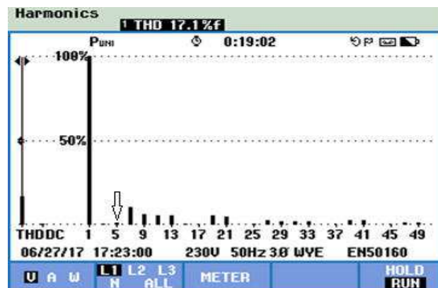
Fig. 7(a) THD results of 5 Level CHB Inverter from Hardware
