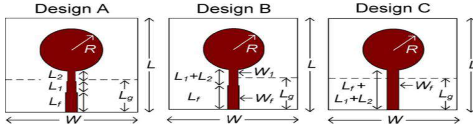
Fig 2: Different 3 designs of circular monopole antennas [1]
