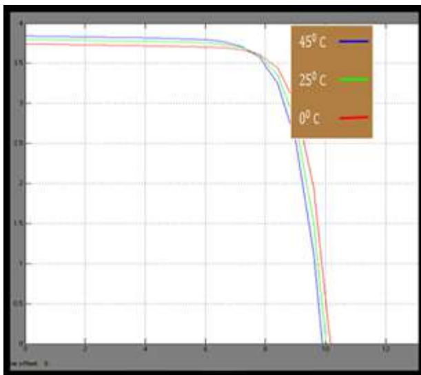
Figure 6: Effect of temperature on I-V curve at insolation 1\text{w/m}^2 .
