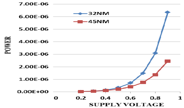
Figure 5. comparison of power as function of supply voltage
