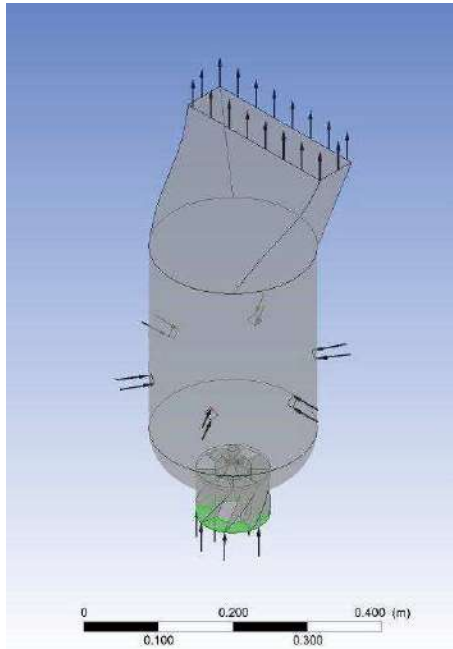
Figure 7: CAD model of Combustion Chamber
