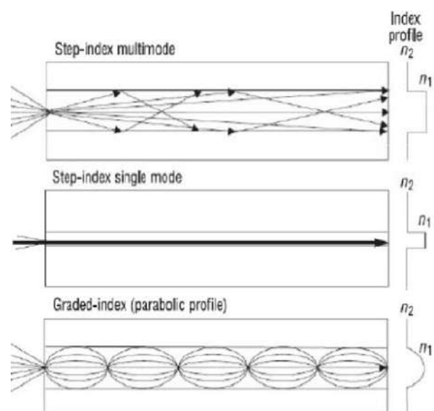
Fig.2. Optical Fiber Modes [6]
