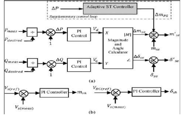
Fig 1: Overall UPFC control system for a damping application. (a) Series VSC control system; (b) Shunt VSC control system.
