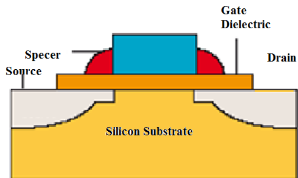
Fig.1: Traditional n-channel MOSFET
