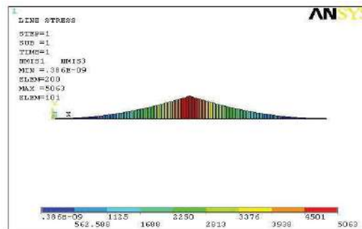
Figure 3 Max. Stress distribution diagram (psi)
