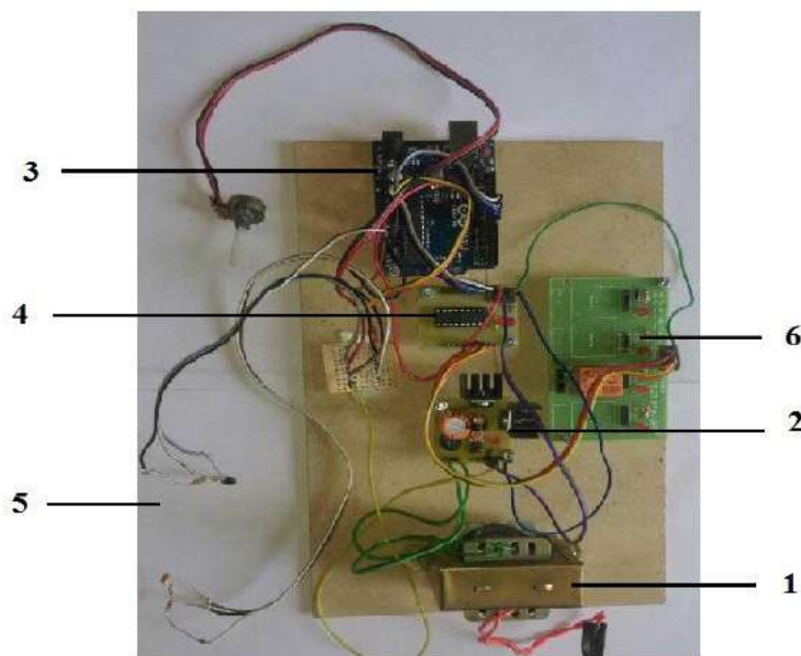
Fig 1.1 Working Model
