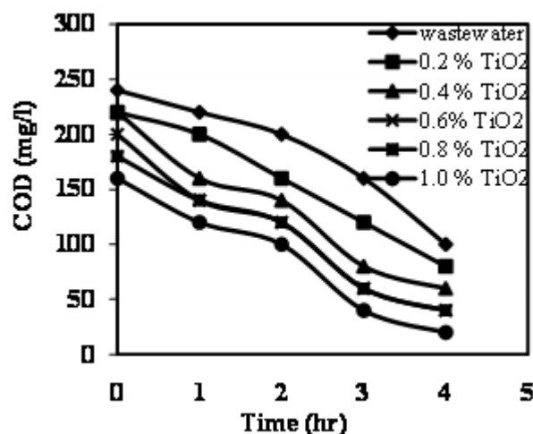
Fig. 2. Effect of catalyst concentration on the COD reduction
