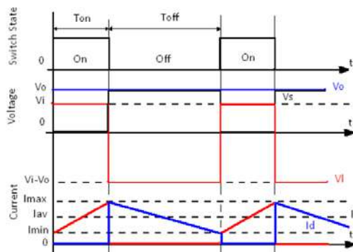
Fig.4. CCM operation of DC-DC converter
