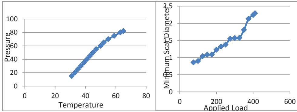
Figure 2. Pressure Vs Temperature (For Oil SAE40) Figure 3. Minimum Scar Diameter (d) mm Vs Applied Load (W) Kg
