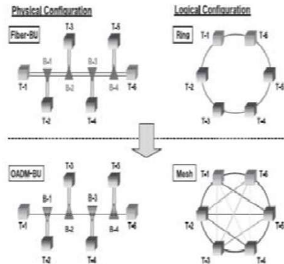
Fig.5. Optical Network Configurations [8]
