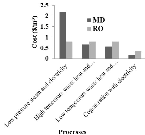
fig.1. Cost comparisons between MD and RO plant based on the type of energy [39]
