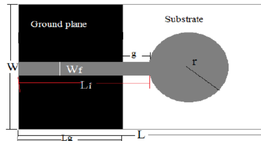
Fig1: Geometry of Printed Circular Monopole Antenna
