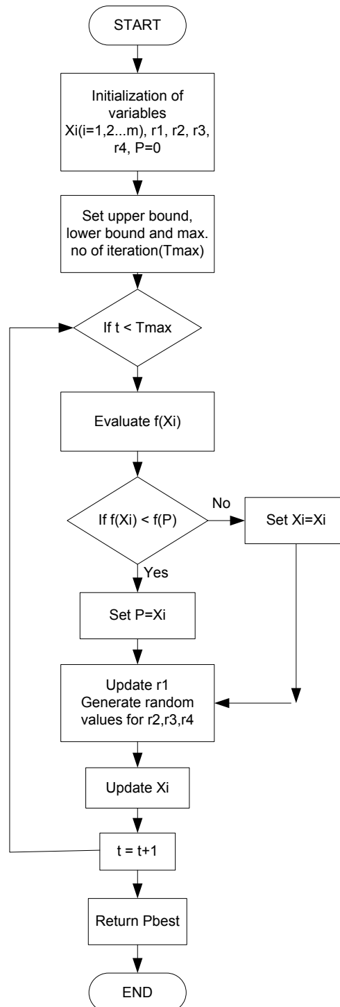
Fig. 3. Flow chart of SCA algorithm
