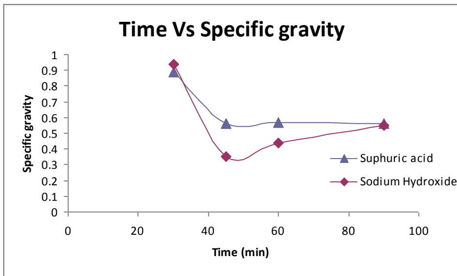
Graph-2 Variation of Specific gravity vs Time
