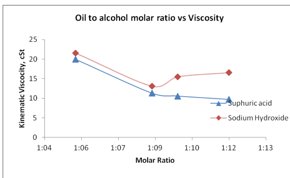
Graph-4 Variation of viscosity vs molar ratio
