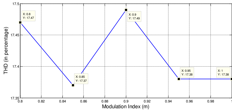
Fig. 5(a). THD verses modulation index for 5 level inverter
