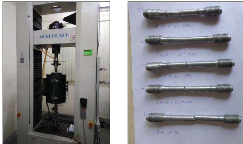
Figure 2. Shimadzu Autograph Machine and tested samples
