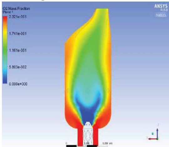
Figure 11: Mass fraction of O_2
