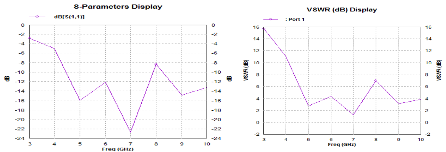
Fig(4): S parameter Graph & VSWR Graph for Design A
