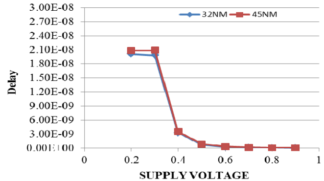
Figure 4. comparison of Delay as function of supply voltage
