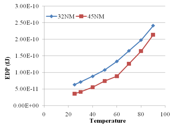
Figure 10. Energy Delay product vs temperature
