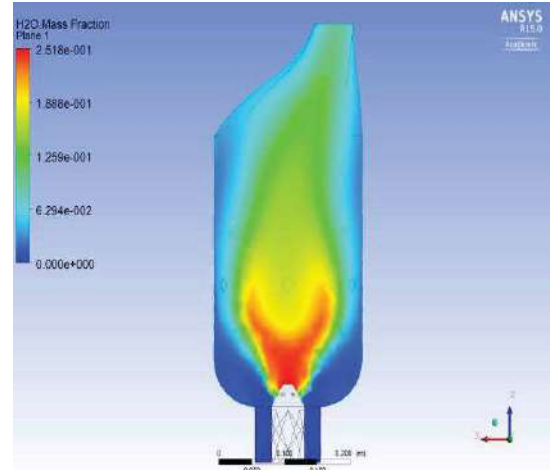
Figure 10: Mass fraction of H_2O
