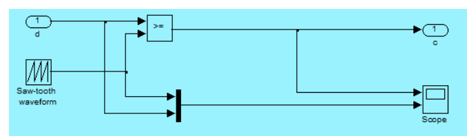
Fig.6. PWM Pulse Generator
