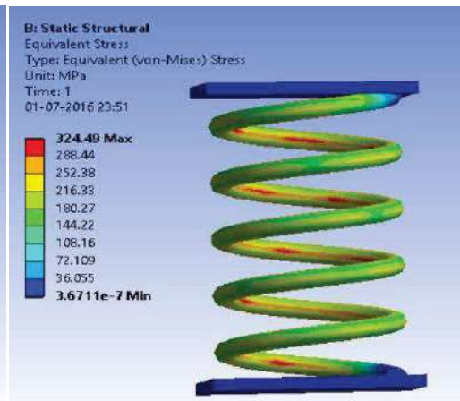
Figure 5. Von Mises Stress on Existing Compression Spring for 500 N Load
