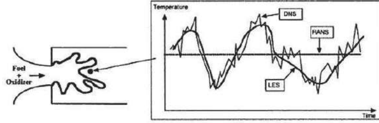
Figure 1: Time evolutions of local temperature for RANS, LES and DNS [16]
