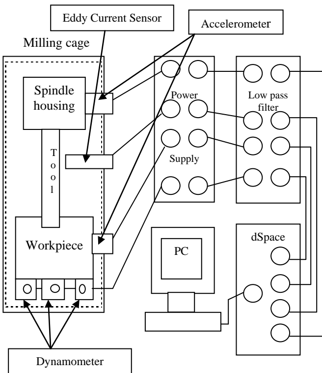
Fig:- Proposed schematic of experimental setup
