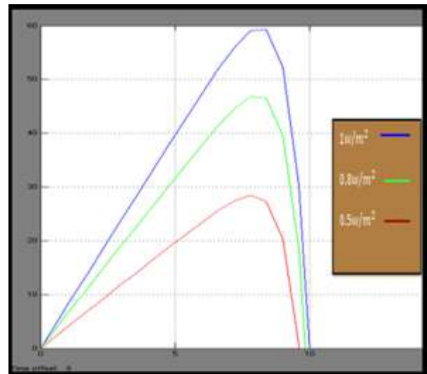
Figure 7: Effect of solar insolation on P-V curve at temperature 25^{\circ} .
