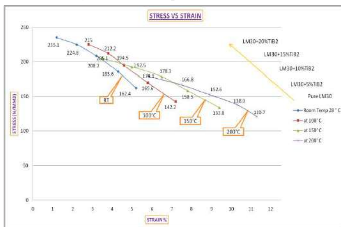
Figure 3. Stress VS % Strain
