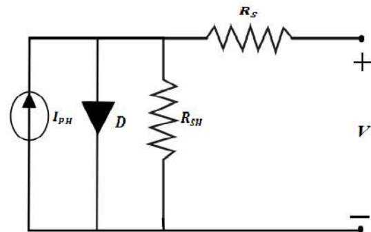
Figure 1: Equivalent model of solar cell
