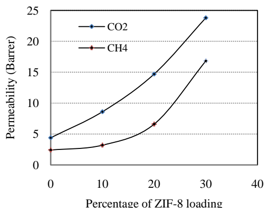
Fig.1. Effect of percentage ZIF-8 loading on single gas Permeabilities of PES–ZIF-8 MMM at 3 bar 30°C
