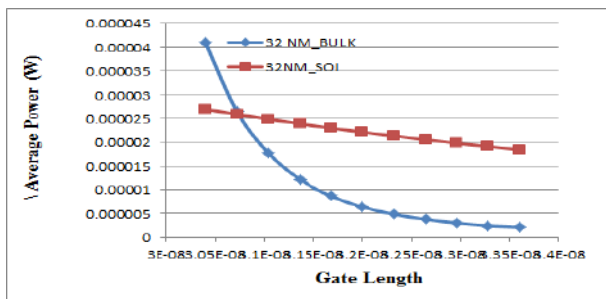
Fig. 11: Average power vs gate length
