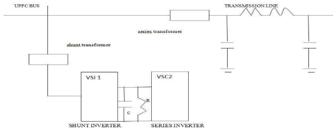
Figure 1: Unified power flow controller configuration
