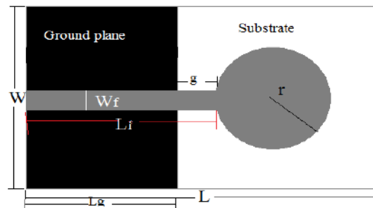
Fig1: Geometry of Printed Circular Monopole Antenna
