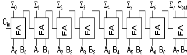
Figure 3. 8-bit Ripple Carry Adder
