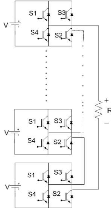
Fig. 1. n-level CHB topology
