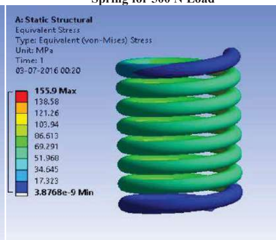
Figure 7. Von Mises Stress on New Compression Spring for 500 N Load
