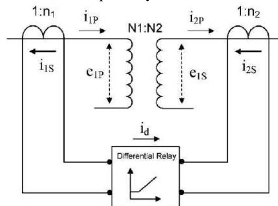
Figure.1. Differential scheme used for the protection of large power transformers
