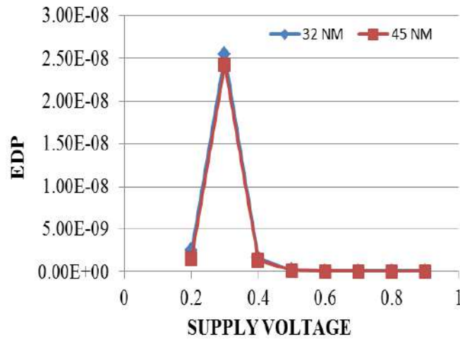
Figure 7. comparison of EDP as function of supply voltage
