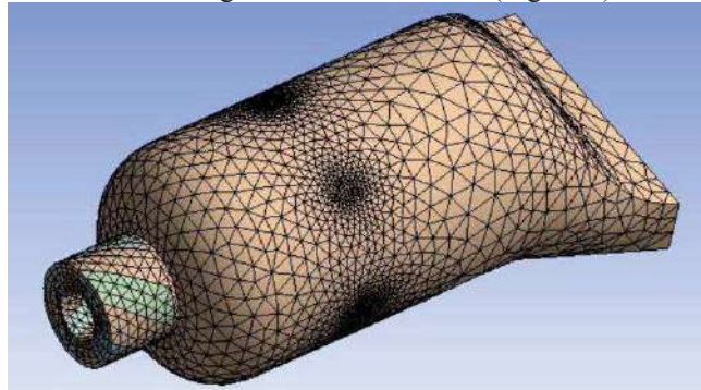
Figure 8: Generated mesh of Combustion chamber
