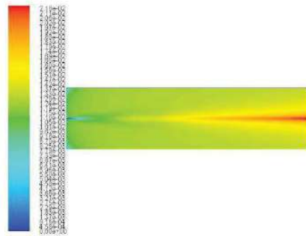
Figure 5: Mass fraction of Pollutant (NOx)
