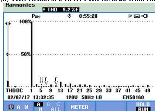
Fig. 7(a) THD results of 5 Level CHB Inverter from Hardware
