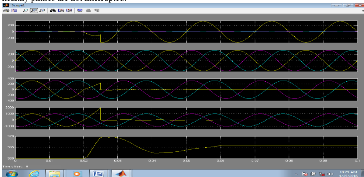
Graph.3.2.(a) Injected voltages, (b) Source voltages. (c) Load voltages. (d) Line currents. (e) DC-link voltage, during the single phase-to-ground downstream fault.
