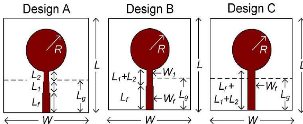
Fig 2: Different 3 designs of circular monopole antennas [1]
