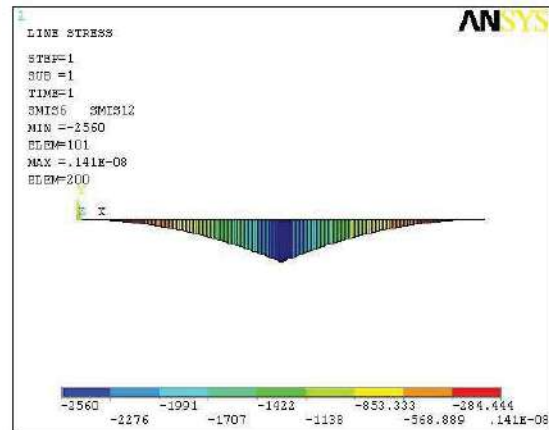
Figure 2 Bending Moment diagram of the beam (lb-in)
