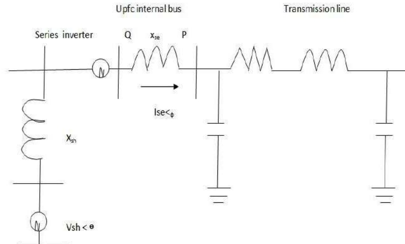
Figure 2:UPFC model
