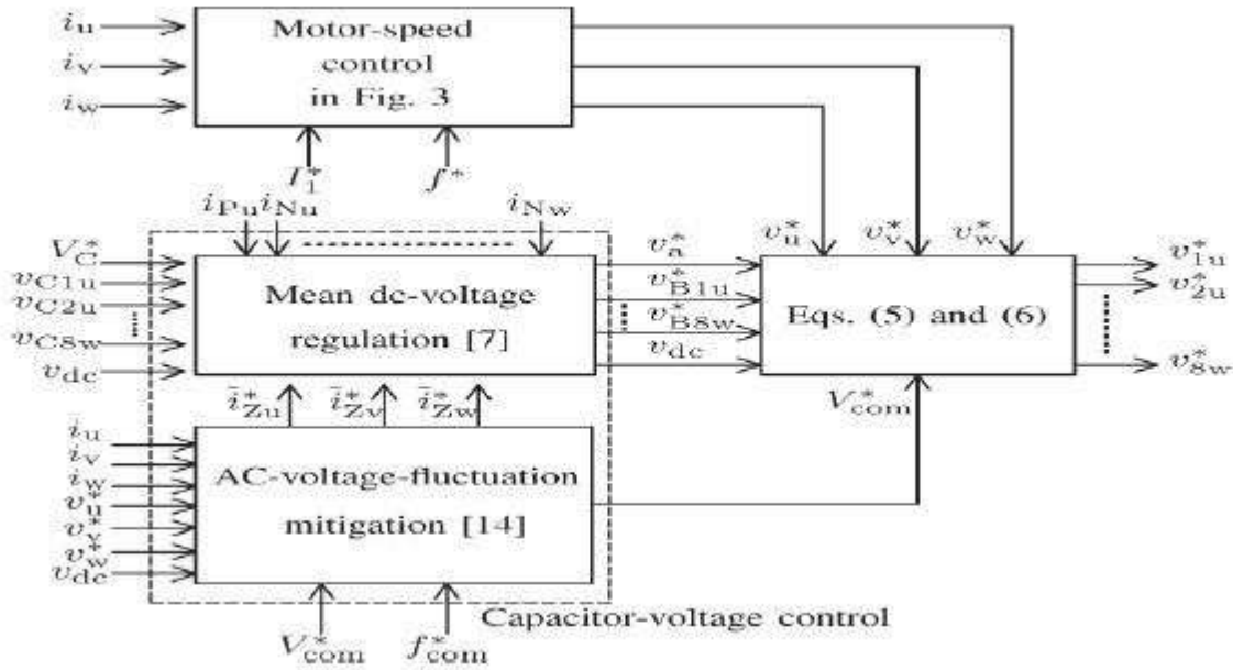
Fig 2: Overall control block diagram for the start-up method
