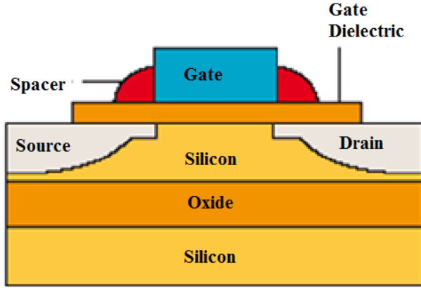
Fig. 2: Silicon-On-Insulator (SOI) MOSFET
