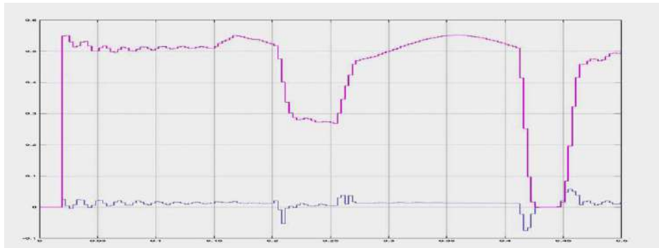
Figure 5: Active and reactive power of series transformer of UPFC
