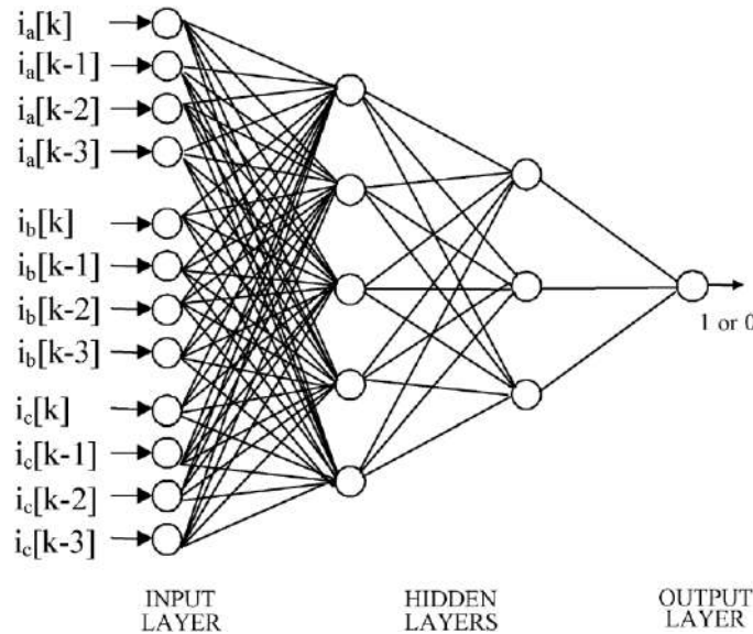
Figure.2. ANN used for pattern recognition
