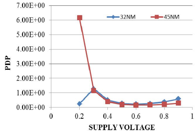
Figure 6. comparison of PDP as function of supply voltage
