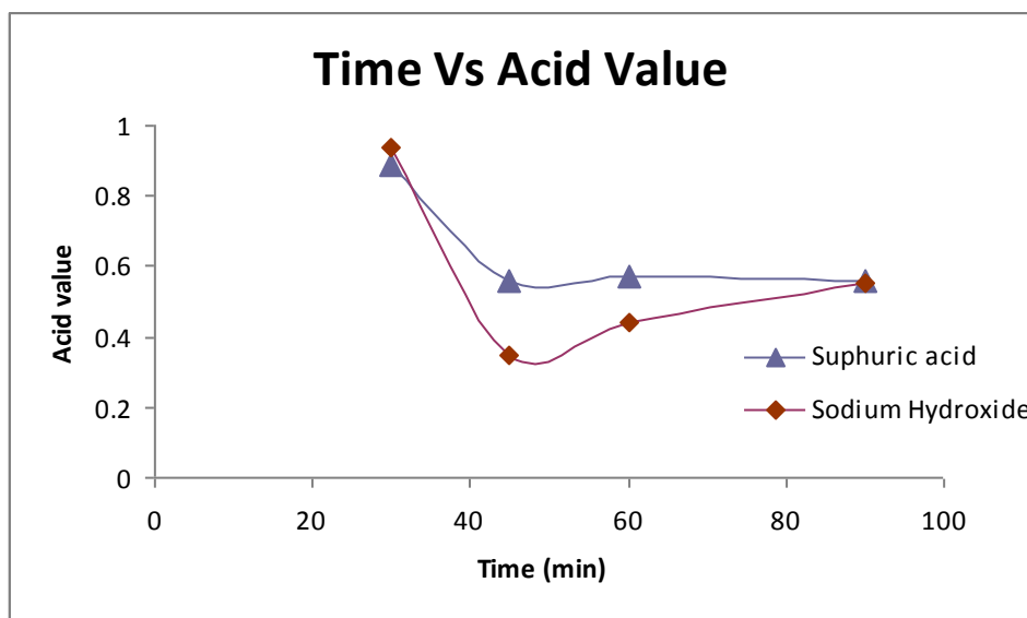
Graph-3 Variation of Acid value vs Time
