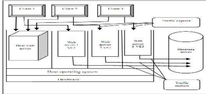
Fig 5: Implementation Architecture
