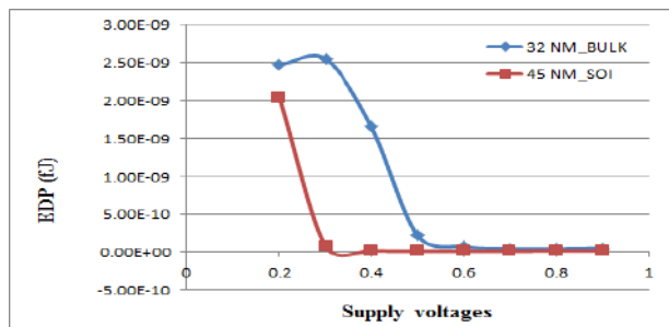
Fig. 6 comparison of EDP as function of supply voltage
