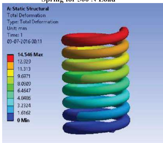
Figure 6. Total Deformation of New Compression Spring for 500 N Load
