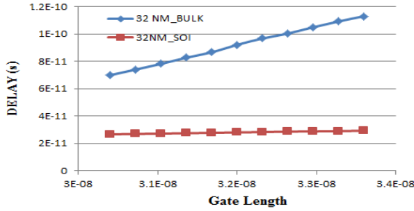
Fig. 10: Delay vs gate length
