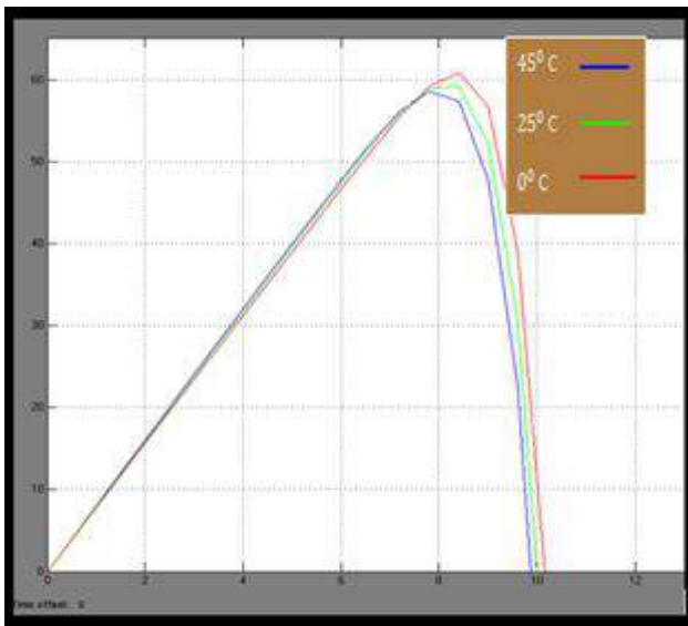
Figure 5: Effect of temperature on P-V curve at insolation 1\text{w/m}^2 .
