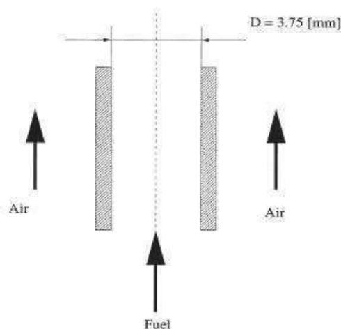
Figure 2: Inlet geometry
