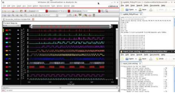
Fig.15. Post Extraction Simulation waveform and digital vector file for Reversible Multiplier
