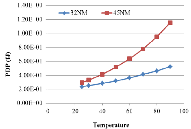
Figure 9. power delay product vs temperature
