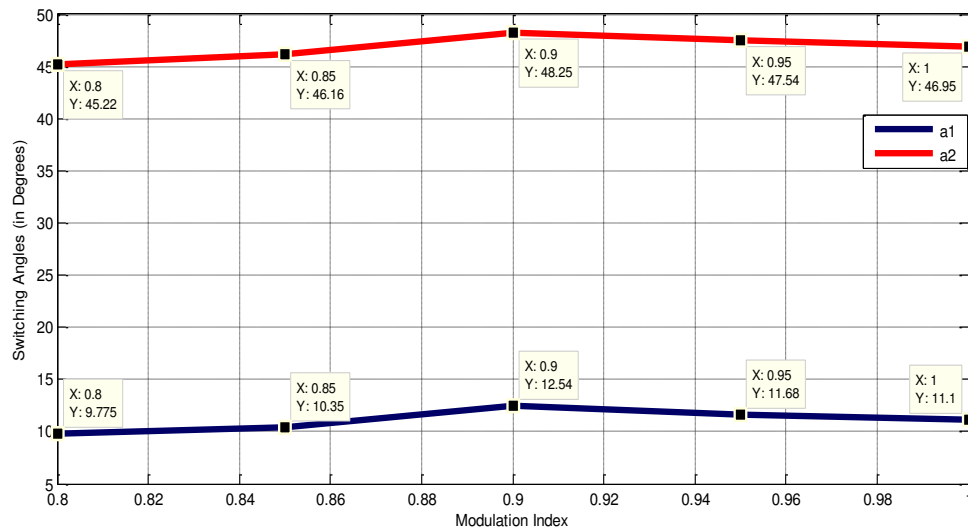
Fig. (4)(a). Modulation index verses switching angles for 5 level CHB
