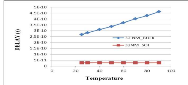
Fig. 7: Comparison of delay as a function of temperature
