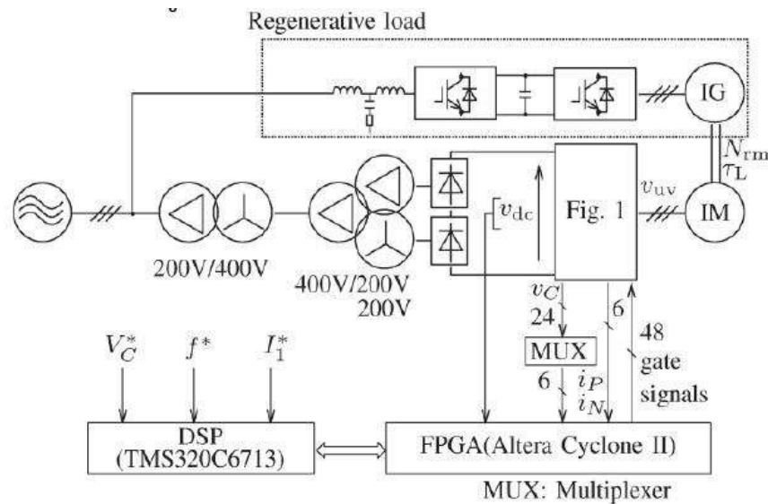
Fig 4: 400-V 15-kW downscaled system used in the experiments
