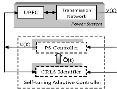
Fig 2: Self-Tuning(ST) controller
