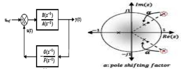
Fig.3 Closed-loop system configuration
