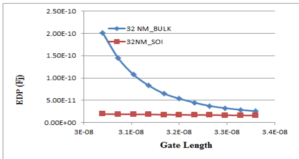
Fig. 12: EDP vs gate length
