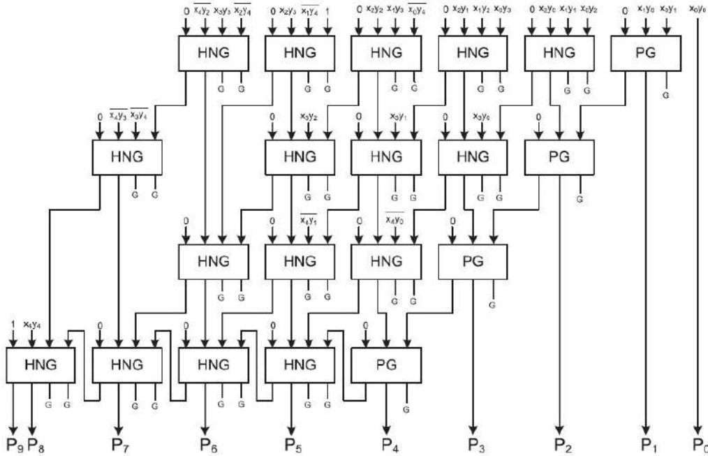
Fig.8. Multi-Operand Addition by Peres and Haghpars-Navi gates
