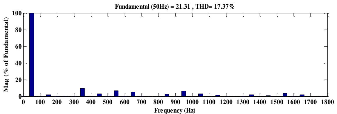
Fig. 6(a). Harmonics analysis using FFT for 5 level inverter
