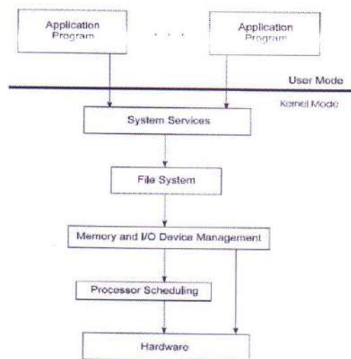
Fig. 1: Layout of operating system
