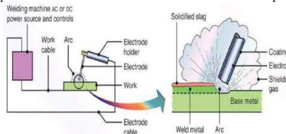
Fig-1.1 SMAW Welding
