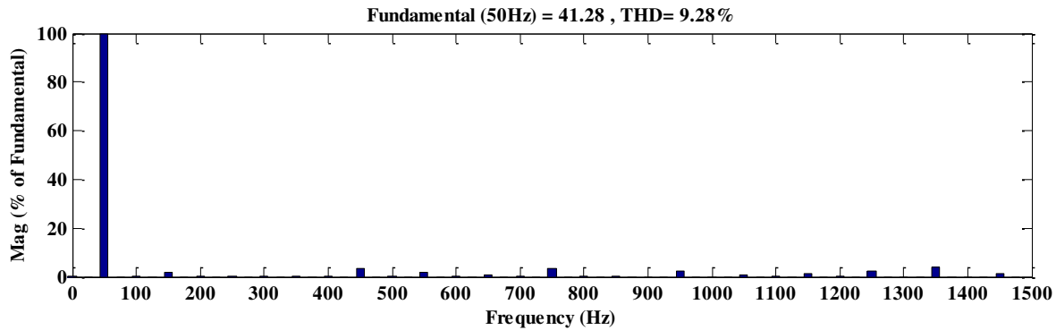
Fig. 6(b). Harmonics analysis using FFT for 9 level inverter
