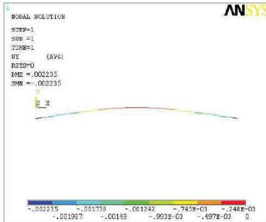
Figure 1 Deformed Shape of the beam (inch)
