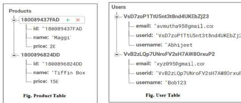
Fig.1.11. Database as a cloud-hosted JSON tree
