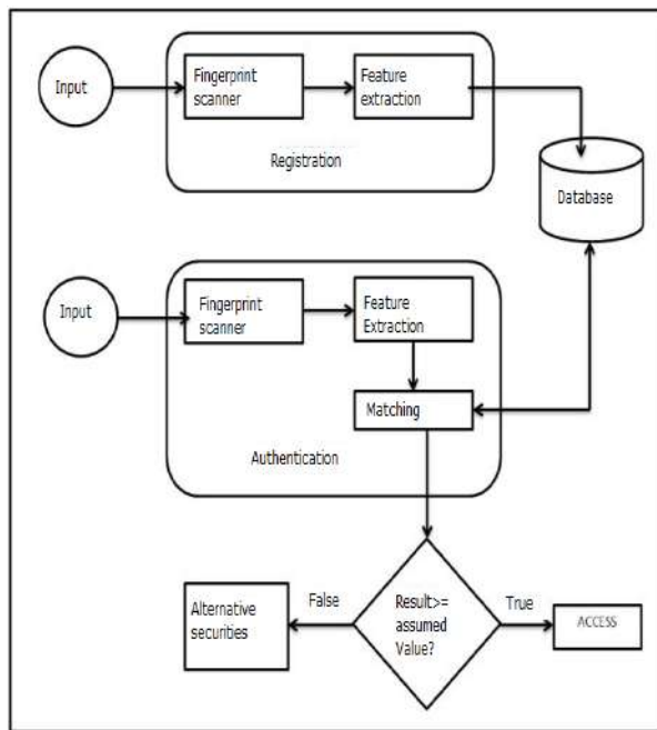
Fig. 4. System Architecture
